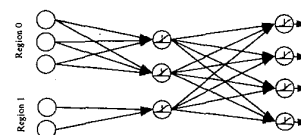
Figure 7. Regions define input-to-hidden neuron connectivity.
