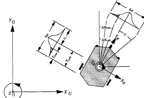
Figure 3. Robot trajectory corrupted by noise.
